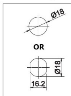
Hole drawing
